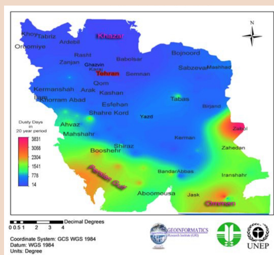
Number of dusty days in Iran over a 20-year period from 1985 to 2005 (Mohamadkhan et al. 2016)
